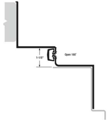
180° Open Position
