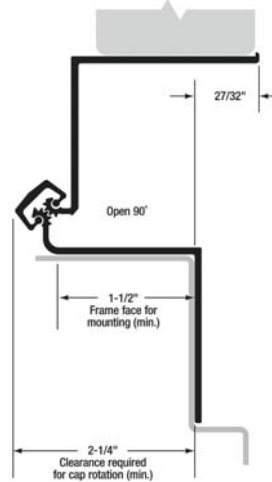
90° Open Position
